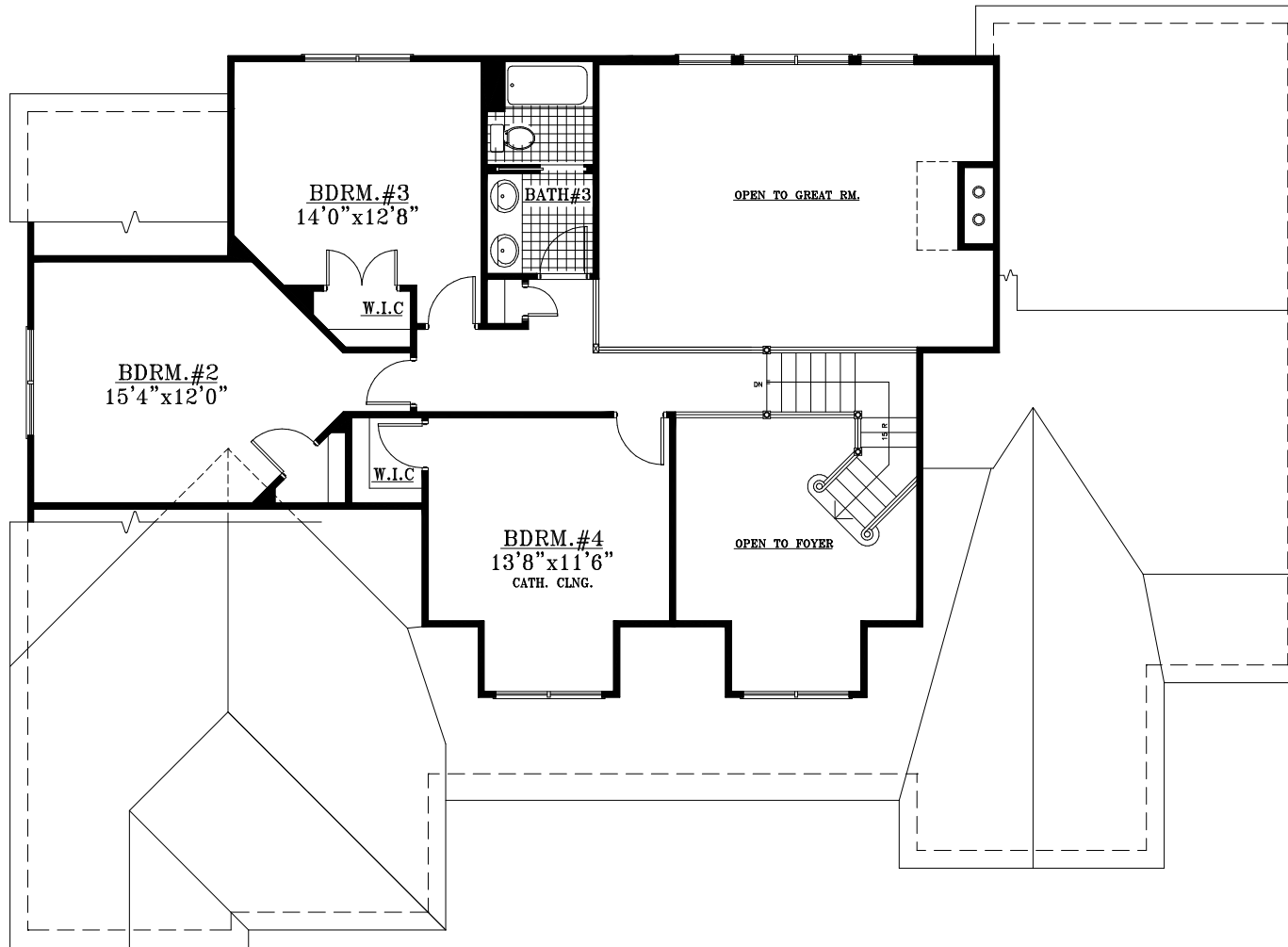
SECOND FLOOR PLAN Not To Scale. Area - 889.00 sq.ft.
